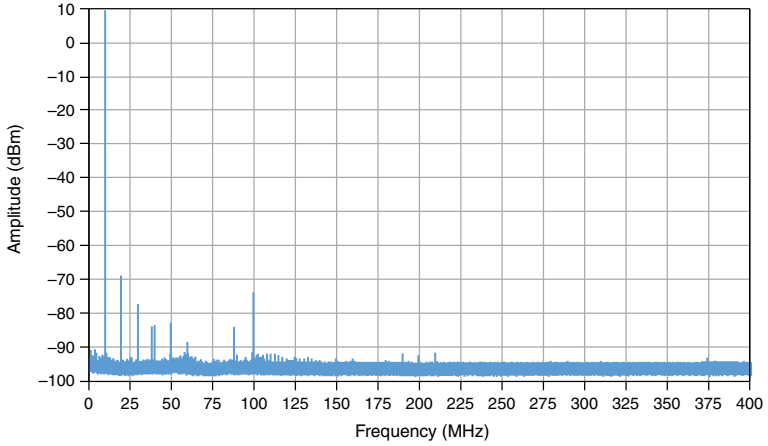
Figure 10. 9.5 MHz and 10.5 MHz Dual-Tone Spectrum 24 , Measured
