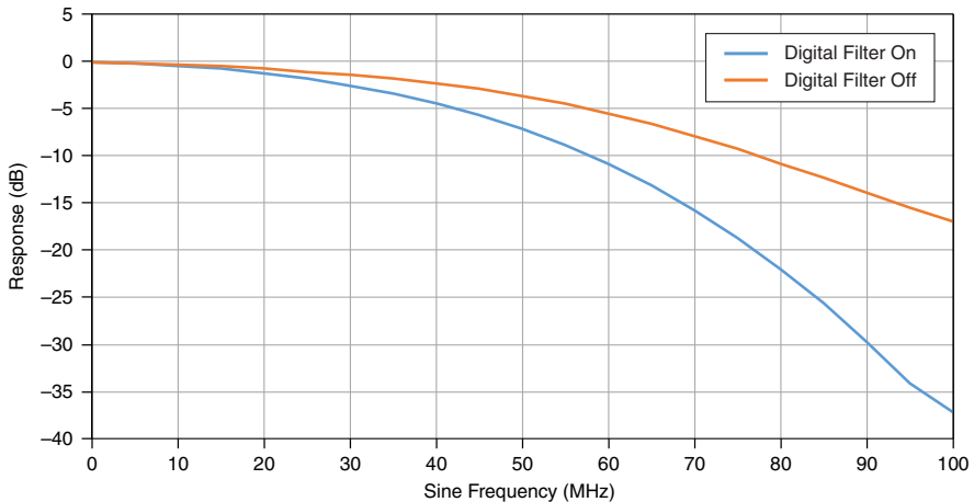
Figure 8. Magnitude Response 22 , Measured
