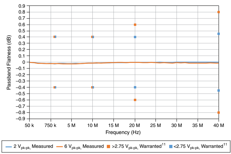
Figure 1. Passband Flatness
